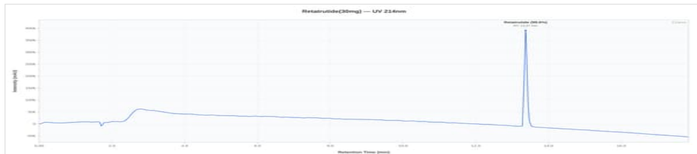
Retatrutide 30mg - 073126: UV Chromatogram
